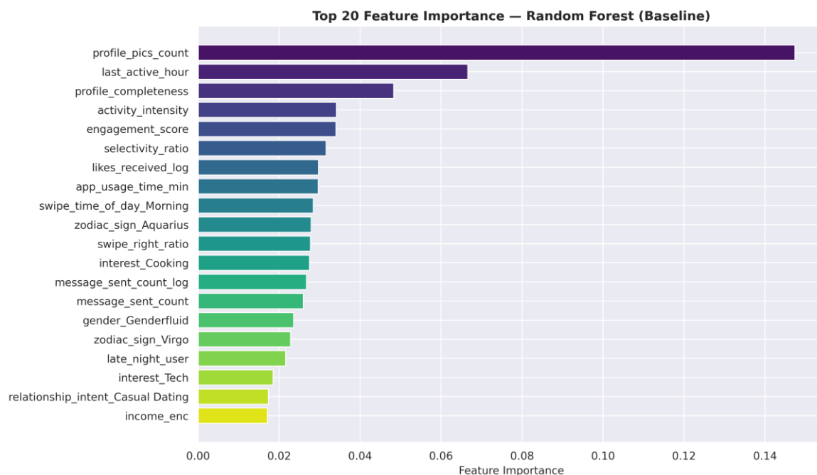
Figure 30: Global Feature Importance Rankings (Tree-based Split Importances)
